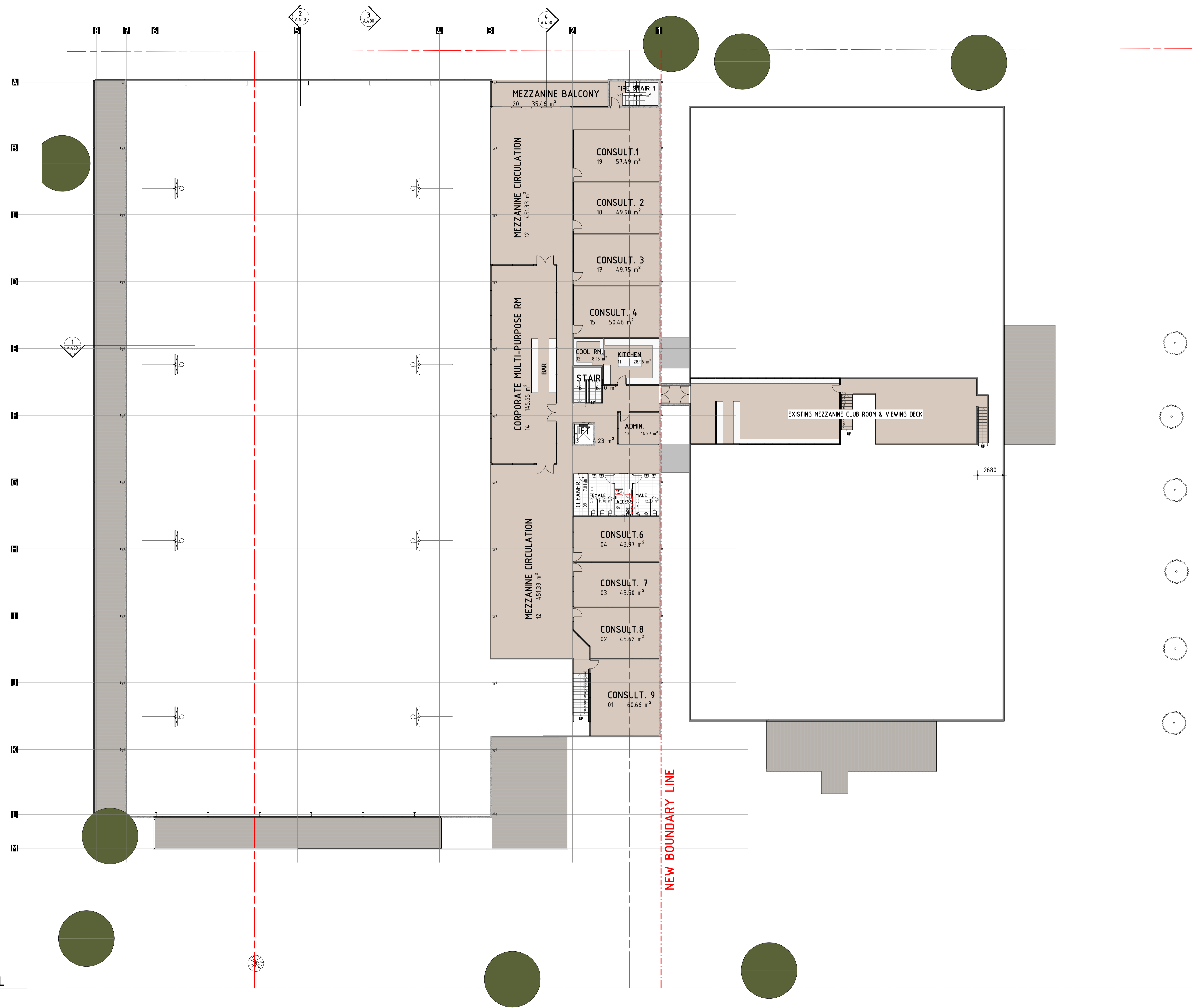
1 MEZZANINE FLOOR LEVEL 1 : 200
